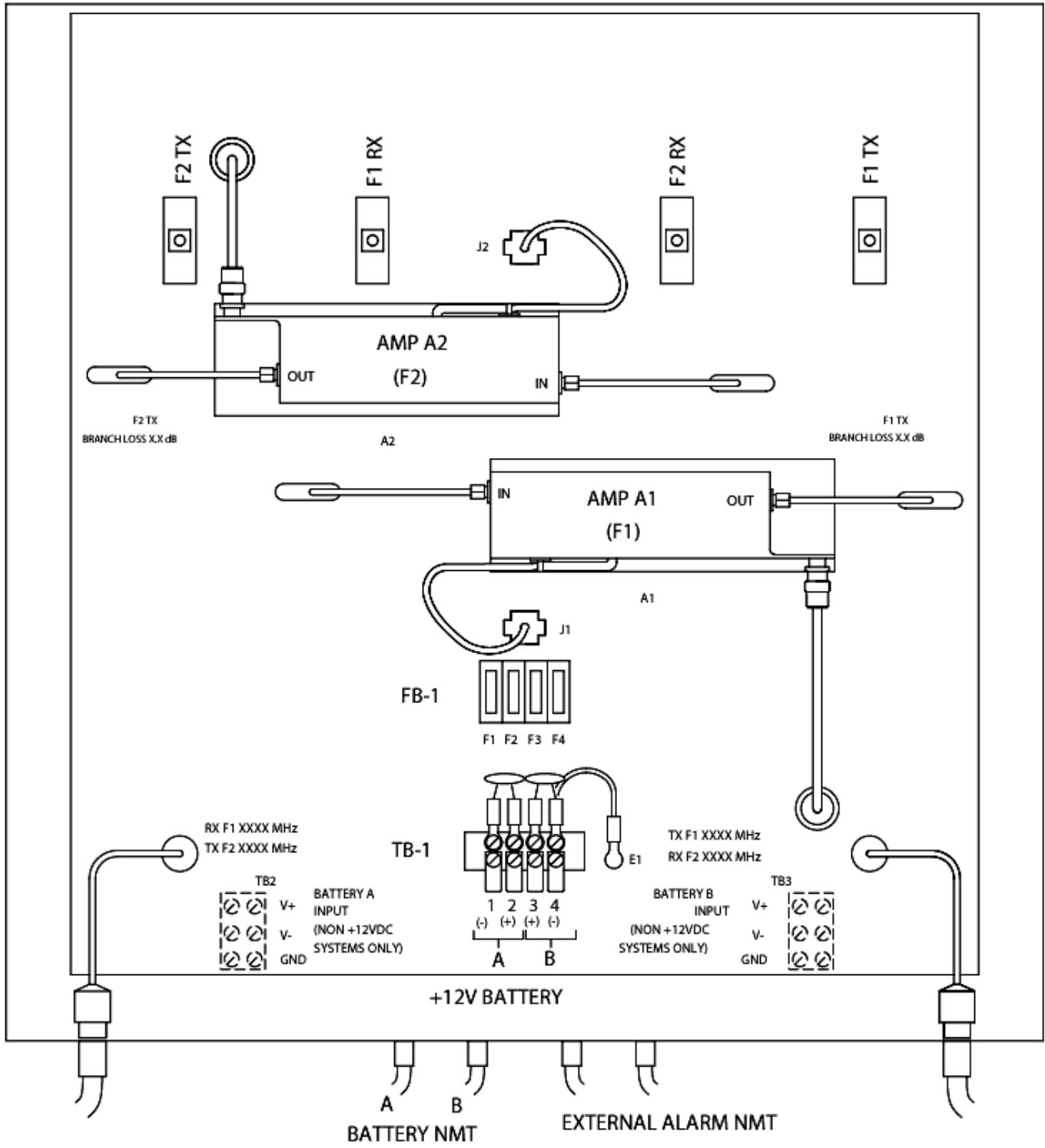
MECHANICAL LAYOUT, DUPLEX
