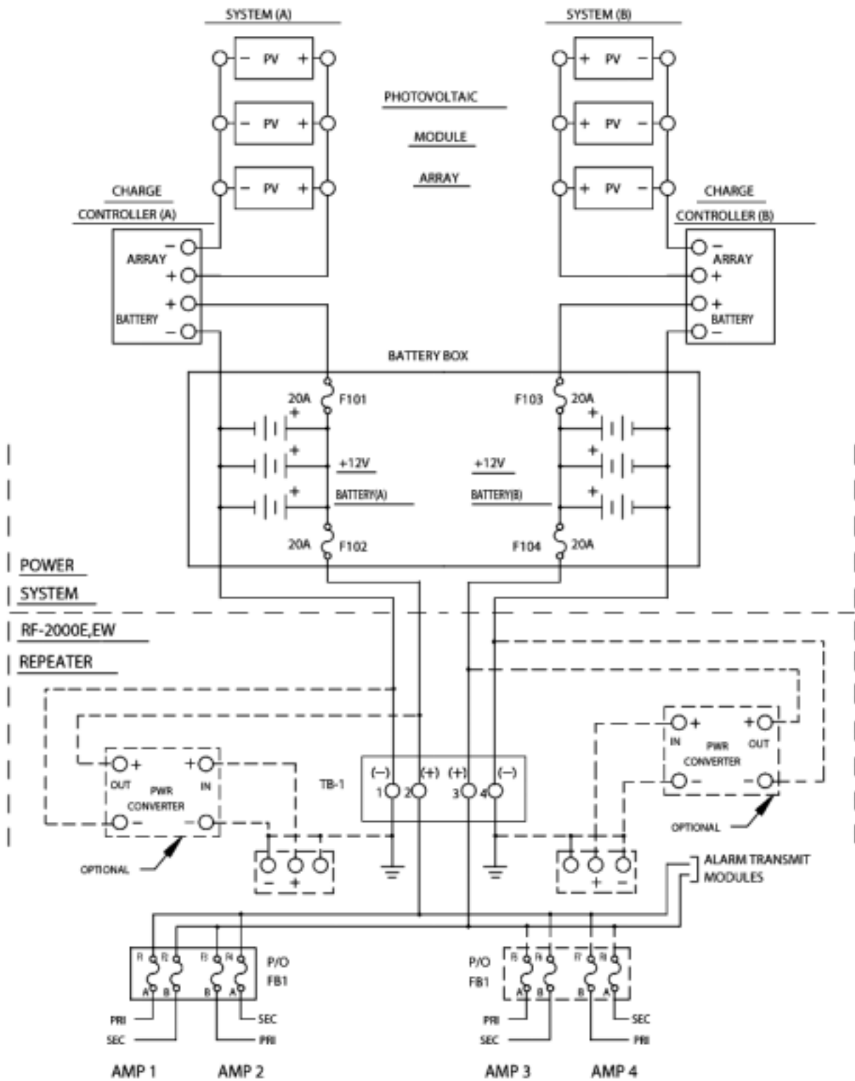
FIGURE 2.8 POWER BLOCK DIAGRAM
