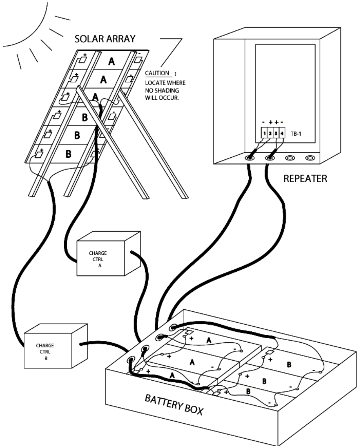
REPEATER POWER WIRING PICTORIAL
