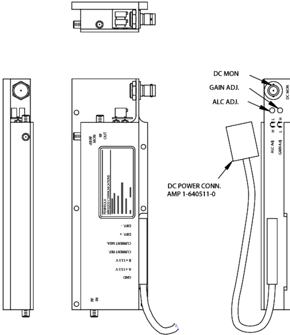
FIGURE 2.7 AMPLIFIER
